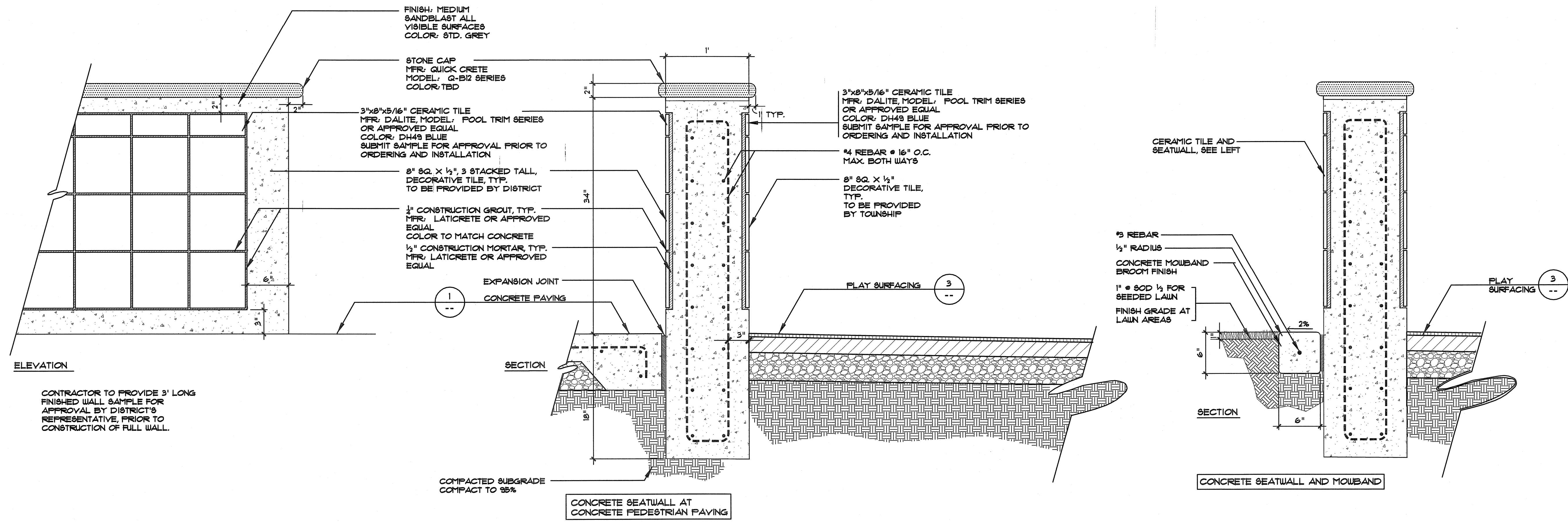
2 CONCRETE SEAT WALL WITH CERAMIC TILES SCALE: 1/2" = 1'-0"
