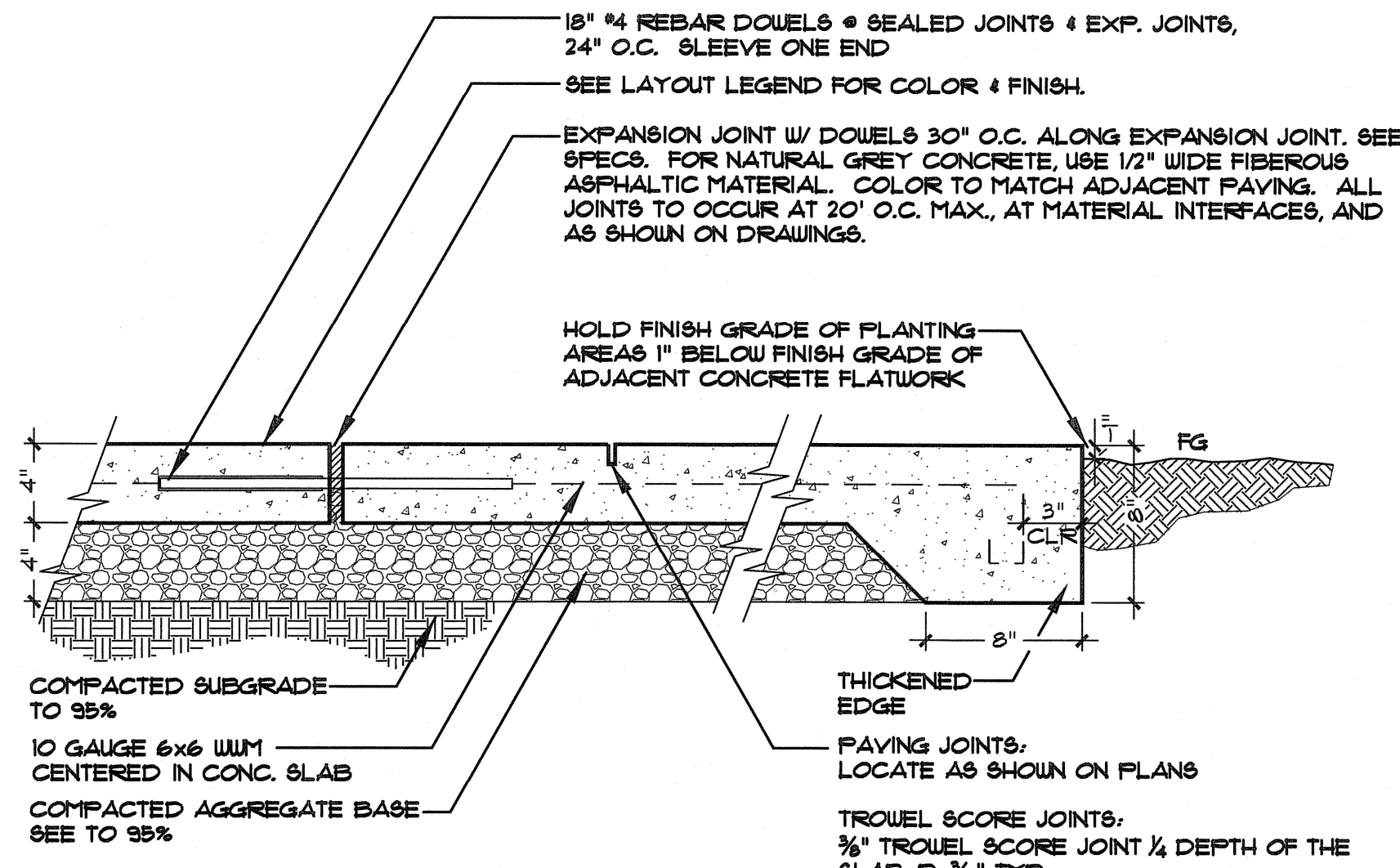
1 CONCRETE PAVING ON GRADE SCALE: 1/2" = 1'-0"
