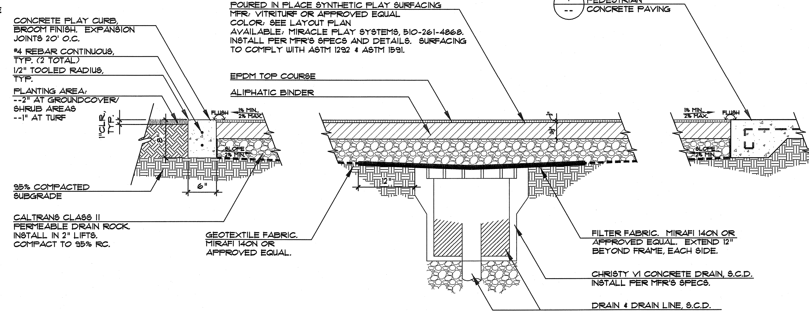
3 SYNTHETIC PLAY SURFACING SCALE: 1" = 1'-0"
